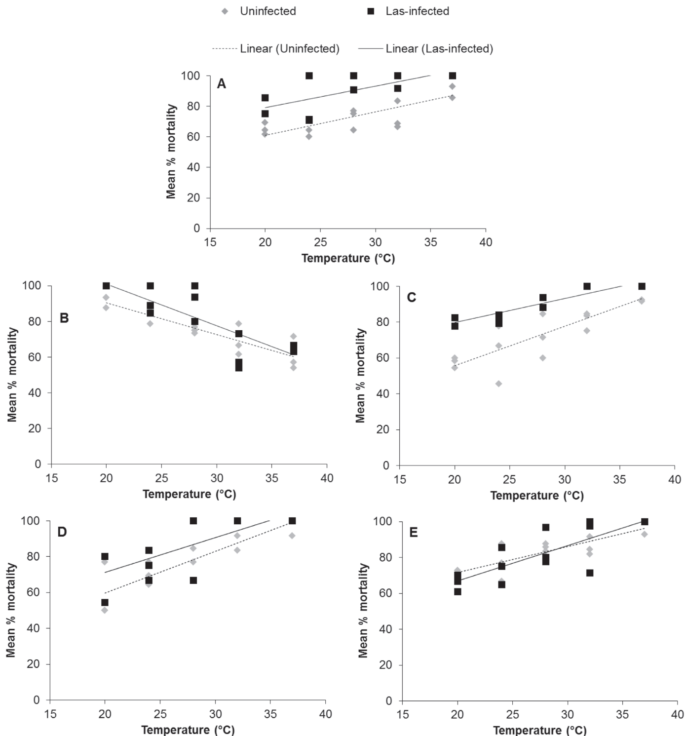
Fig. 3. Correlations between mean percentage mortality of Diaphorina citri and temperature for field-collected and uninfected D. citri and field-collected and Candidatus Liberibacter asiaticus -infected D. citri , when exposed to chlorpyrifos (A), fenpropathrin (B), imidacloprid (C), thiamethoxam (D), and spinetoram (E).
