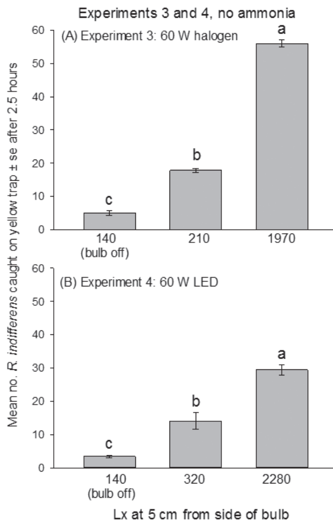
Fig. 2. Mean numbers \pm SE of Rhagoletis indifferens flies caught on sticky yellow traps with no ammonia lure at different light intensities (lx) shown along the x-axis: (A) experiment 3, 60 W halogen bulb and (B) experiment 4, 60 W LED bulb. Light intensities inside test cage were 90 to 250 lx. Maximum number of flies was 60. Means with same letters are not significantly different ( P > 0.05 , Tukey's HSD test).
