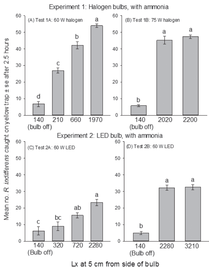
Fig. 1. Mean numbers \pm SE of Rhagoletis indifferens flies caught on sticky yellow traps with ammonia lure at different light intensities (lx) shown along the x-axis: experiment 1: (A) test 1A, 60 W halogen bulb; (B) test 1B, 75 W halogen bulb; experiment 2: (C) test 2A, 60 W LED bulb; (D) test 2B, 60 W LED bulb. Light intensities inside test cage were 90 to 250 lx. Maximum number of flies was 60. Means with same letters are not significantly different ( P > 0.05 , Tukey's HSD test).
