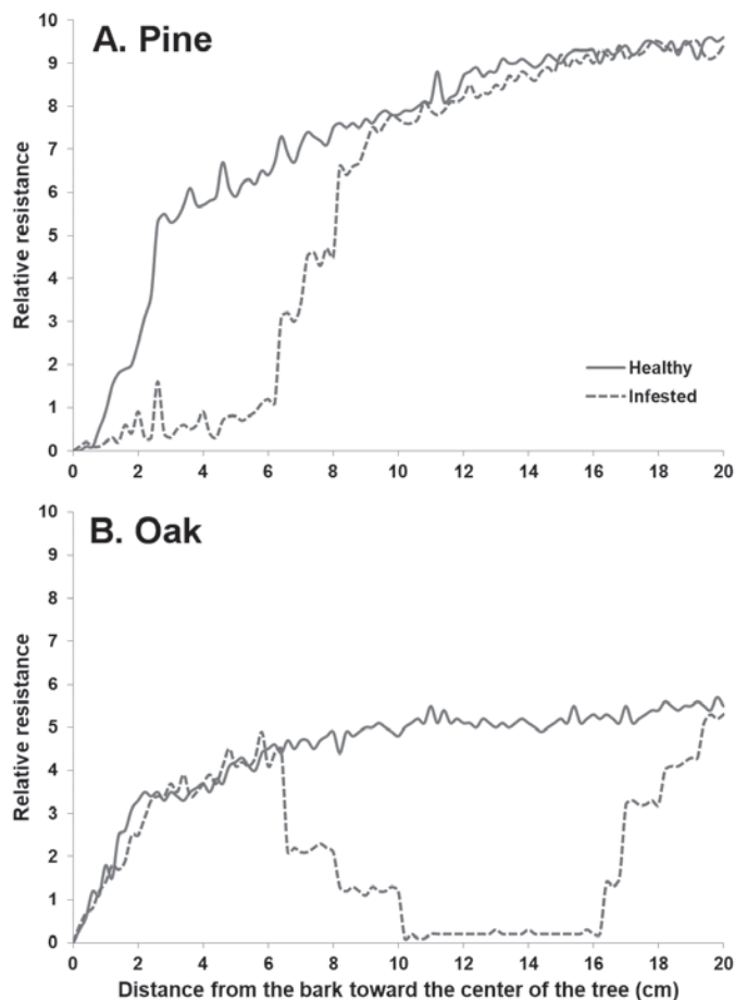
Fig. 9. Relative resistance (density) of the wood on different live trees, categorized as healthy or infested with Coptotermes gestroi . Each line represents the average resistance value obtained from the resistograph, from 3 trees per category, with 3 subsamples per tree ( n = 3 ). (A) Pine trees, (B) oak trees. Infested pine trees reveal damage right underneath the bark, while infested oak trees reveal a cavity at the center of the trunk. The “step” effect on the lines resulted from the average of 3 different trees, with different level of termite damage.
