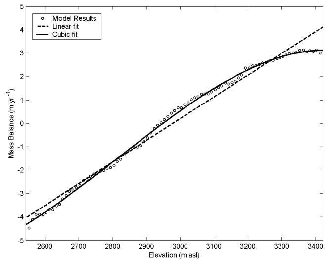
FIGURE 2. Mass-balance/elevation profile for the standard run, averaged over the glacier surface by 10-m elevation-change bands. Open circles: model results; dashed line: best-fit linear relationship; solid line: best-fit cubic relationship.
