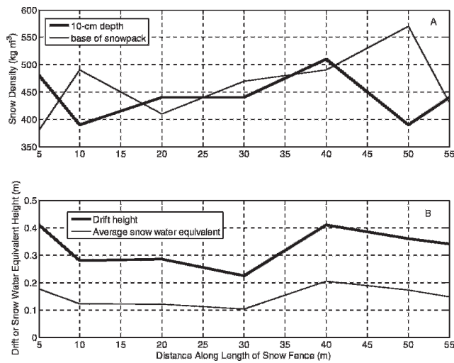
FIGURE 9. (A) Snow density measured near the surface (10-cm depth) and base of the snowdrift 0.50 m from the start of the drift downwind of the structural fence. (B) Mean drift height and snow water equivalent (expressed as a height) using the mean density at each location as shown in panel (A).
