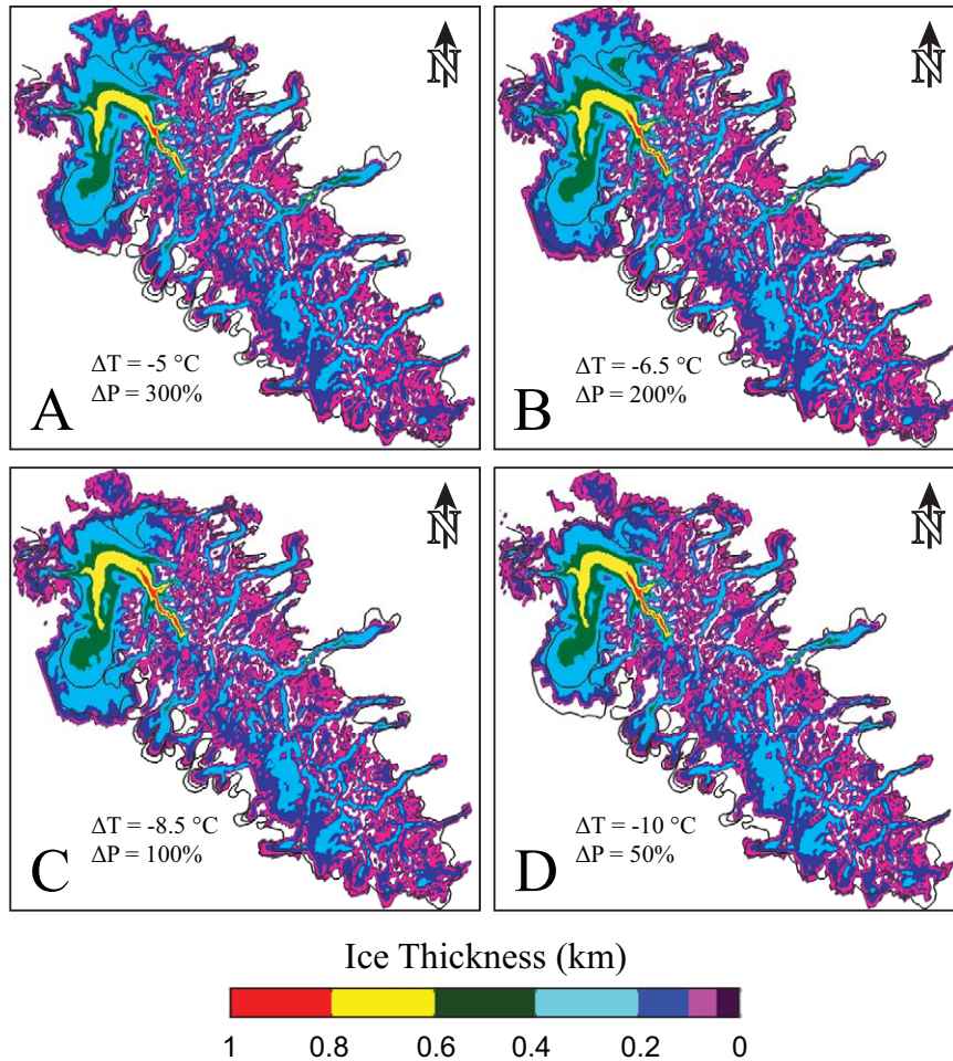
FIGURE 7. Ice thickness reconstructions for (A) T = -5 °C, P = 300\% ; (B) T = -6.5 °C, P = 200\% ; (C) T = -8.5 °C, P = 100\% ; and (D) T = -10 °C, P = 50\% . Black outline denotes ice cap margin inferred from moraines. Areas in which there are two lines show Pinedale (inboard) and Bull Lake (outboard) margins. The greatest difference in ice thickness between the simulations is found over the Green River outlet glacier. Note the linear margins along the western side of the latter glacier in B and C delineate the edge of the model domain. Last Glacial Maximum (LGM) limits were inferred from Google Earth™ imagery with guidance from geomorphological interpretations in Gosse et al. (1995a, 1995b), and from unpublished fieldwork carried out in the summers of 2008 and 2009. In color online.
