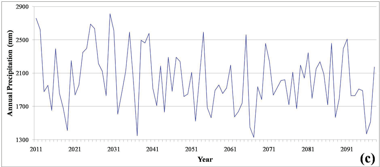
FIGURE 6. Projected temperature and precipitation for Lidder watershed (2010–2098).
