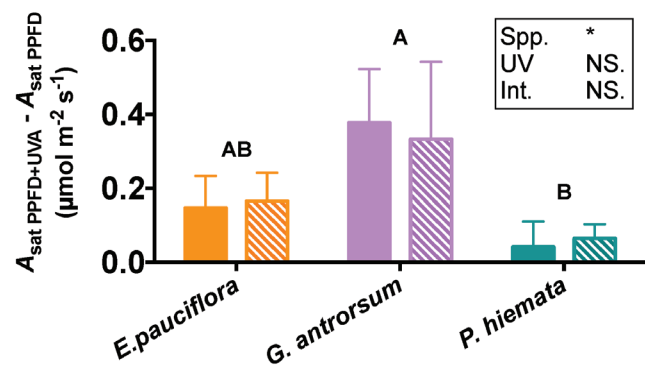
FIGURE 3. Effect of inclusion of UVA wavelengths on the light saturated photosynthetic rate ( A_{sat} ) for E. pauciflora , G. antrorsum , and P. hiemata . Filled bars represent the full sunlight treatment; dashed bars represent the UV exclusion treatment. Values are means \pm SEM ( n = 15 ). Asterisks indicate significantly different means (* P < 0.05 , ** P < 0.01 , *** P < 0.001 ) between light treatments, within species; upper-case letters denote significantly different means between species identified by Fisher's LSD test ( P < 0.05 ).
