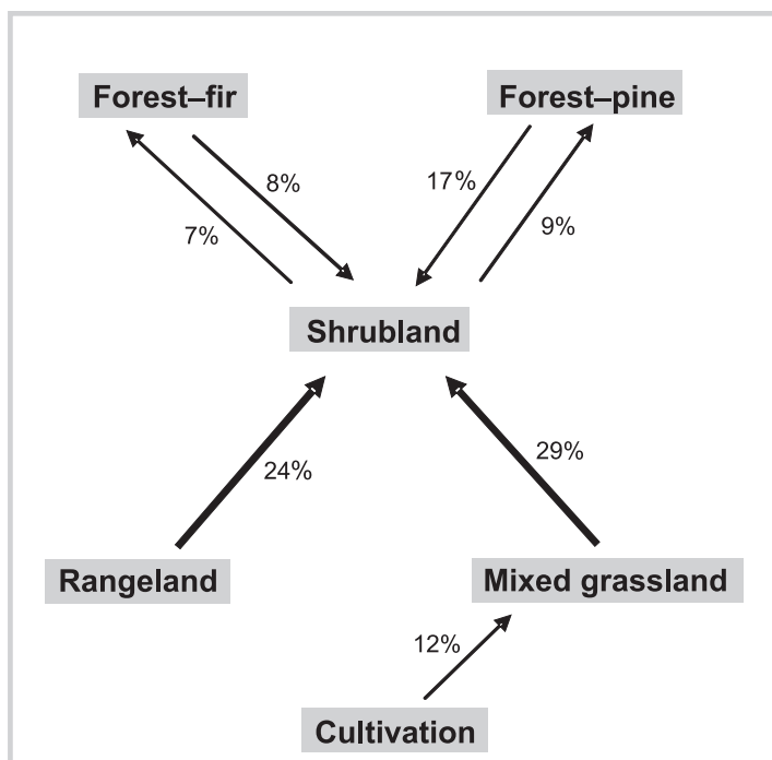
FIGURE 6 Diagrammatic summary of 1990 to 1999 LULC conversions. % = proportion of the 1990 total for each class; conversions under 5% not shown; bolded arrows highlight more than 20% conversion.
