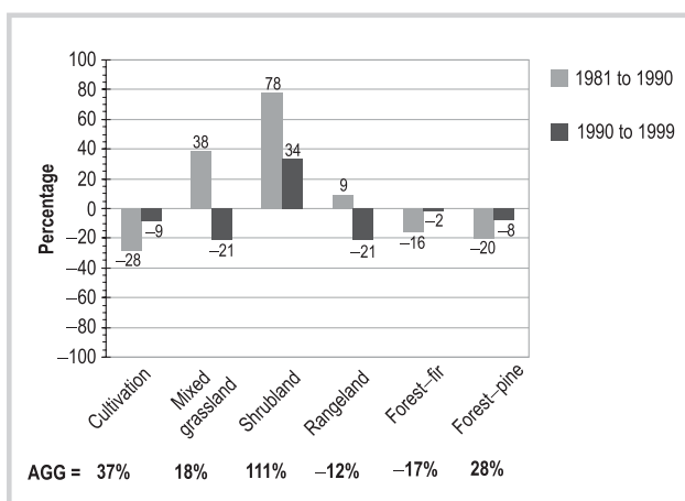
FIGURE 4 LULC rate of change within each class. % calculated by dividing the difference by the base year for each class; figures are rounded; AGG represents the "aggregate change" from 1981 to 1999.
