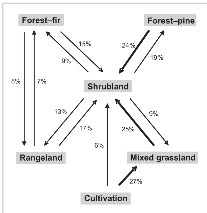
FIGURE 5 Diagrammatic summary of 1981 to 1990 LULC conversions. % = proportion of the 1981 total for each class; conversions under 5% not shown; bolded arrows highlight more than 20% conversion.
