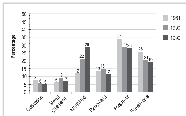
FIGURE 3 LULC proportions for 1981, 1990, and 1999. % = amount of each LULC class as a proportion of the total LULC area for that year, excluding the mask.
