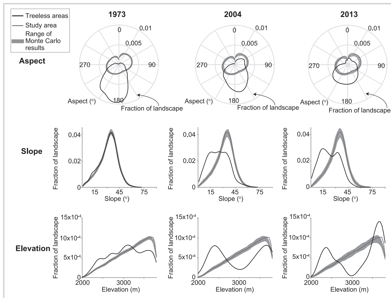
FIGURE 3 Monte Carlo simulation results; distribution of topographic parameters for the entire study area and of environmental parameters for land cleared during 1973, 2004, and 2013. From left to right, data from 1973, 2004, and 2013. From top to bottom, aspect, slope, and elevation data.
