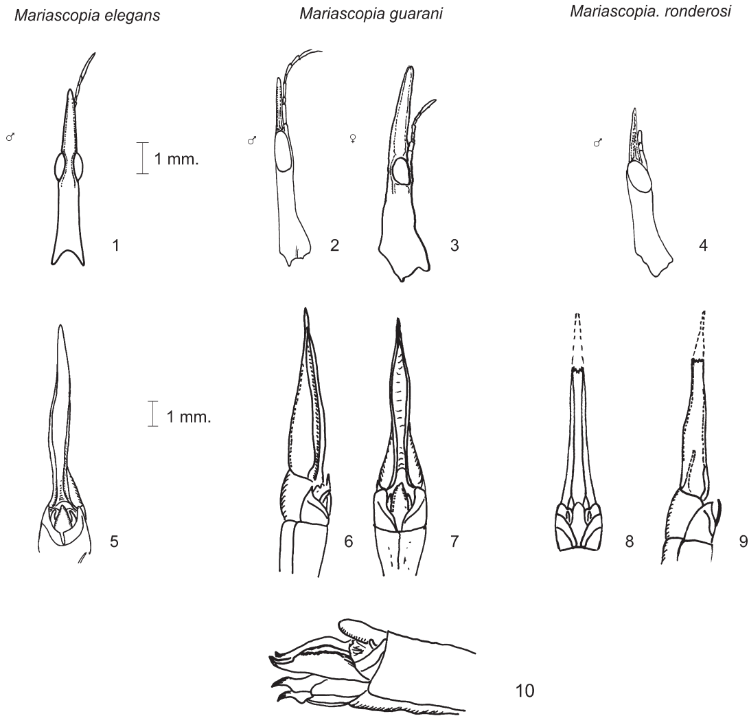
Figs 1-10. External morphological characteristics of Mariascopia species.
