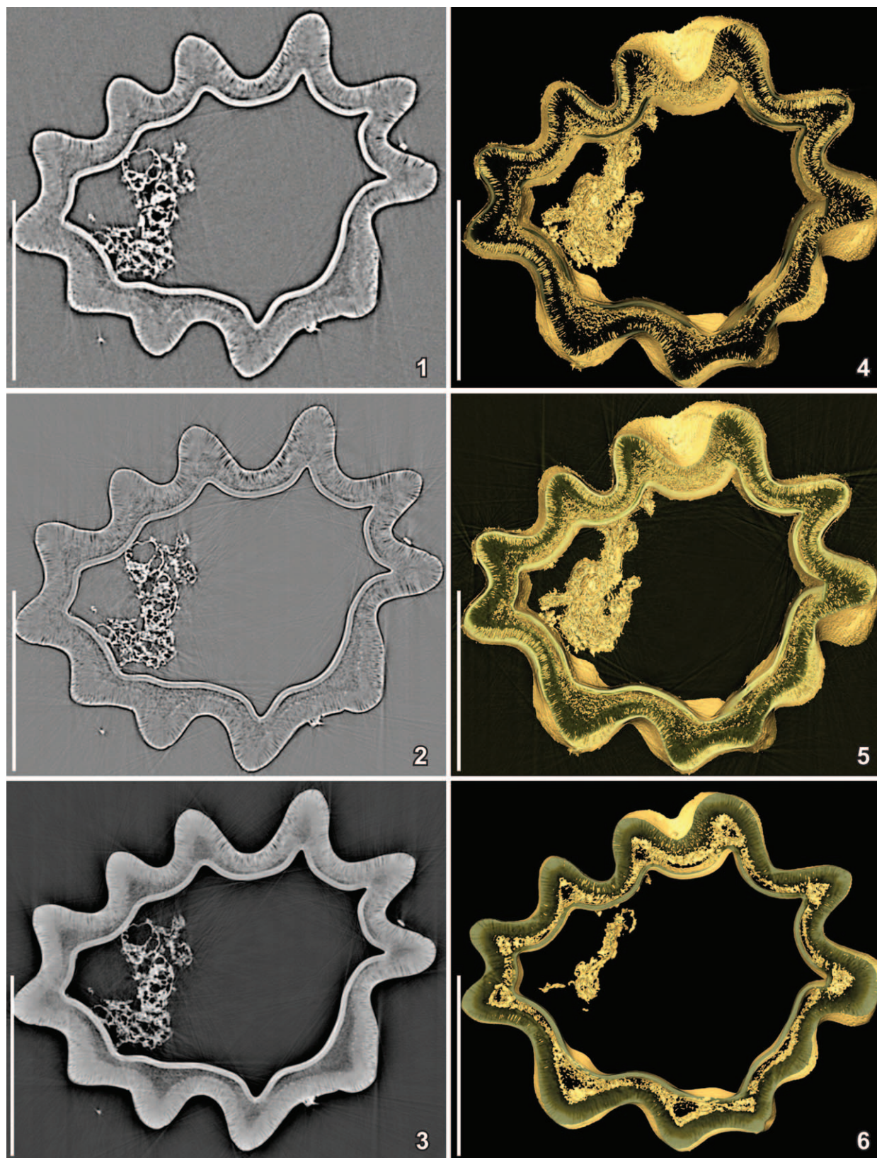
FIGURE 3—SRXTM images of the megaspore Arcellites sp. (S171531) from the Early Cretaceous Torres Vedras locality, Portugal; dataset acquired using a 20 \times objective and 20 \mu m thick LAG:Ce scintillator (voxel size 0.37) at 10 keV (1) and a 40 \times objective with a 5.9 \mu m thick LSO:Tb scintillator (voxel size 0.1625) at 10 keV (2–6); images in 1, 2 and 4, 5 have been reconstructed uniquely exploiting absorption contrast and pure edge-enhancement. Images in 3, 6 were obtained using simple phase retrieval (Paganin et al., 2002), but with the subsequent addition of the high frequency component of the original data to minimize loss in spatial resolution inherent in phase retrieval. 1–3, 2-D reconstructions of a transverse section through the body of the megaspore showing wall ultrastructure composed of a thin inner, almost solid, uniform layer, a middle granular-fibrous layer of uneven thickness, and an outer layer penetrated by very fine canals; note difference in resolution between 1 originating from a tomographic volume obtained with a 20 \times objective and a 20 \mu m thick LAG:Ce screen, and
