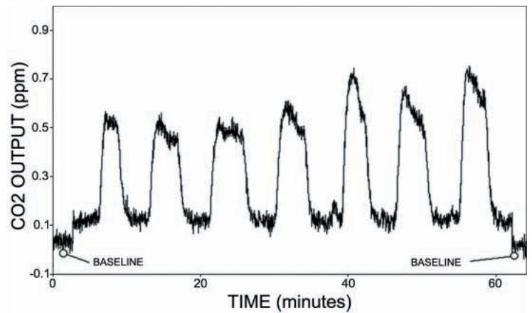
Figure 1. Typical CO 2 emission data by a 6.02 mg pseudoscorpion, Garypus californicus , at 15 °C. Flow rate was 20 ml min -1 .
