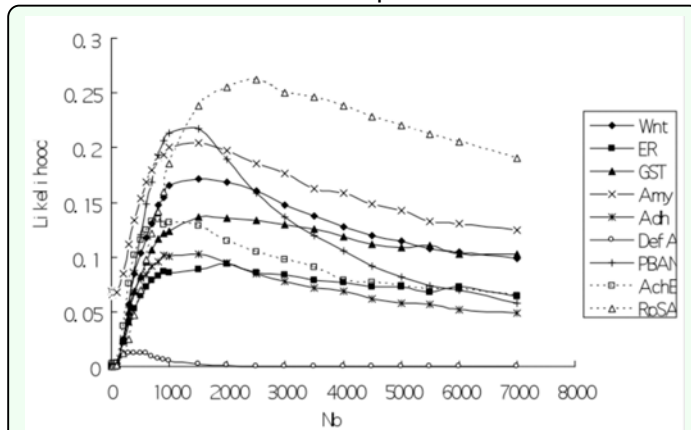
Figure 2. Likelihood curves of 9 loci using the number of segregating sites ( S ) as fit standard with d=1000 . High quality figures are available online.
