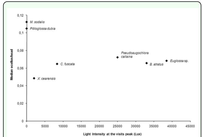
Figure 5. Relationship between the ratio of the diameter of the median ocellus to head width and light intensity (Lux) during the period of peak bee visits to Cambessedesia wurdackii flowers in an area of campo rupestre vegetation in Mucugê, Bahia State, Brazil. High quality figures are available online.
