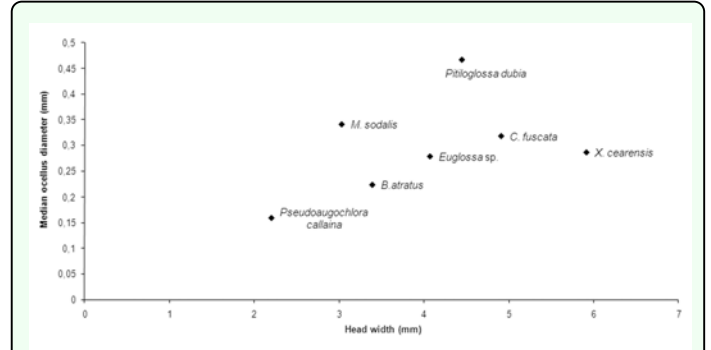
Figure 4. Relationship between the diameter of the median ocellus (mm) and head width (mm) of the bees visiting Cambessedesia wurdackii flowers in an area of campo rupestre vegetation in Mucugê, Bahia State, Brazil. High quality figures are available online.
