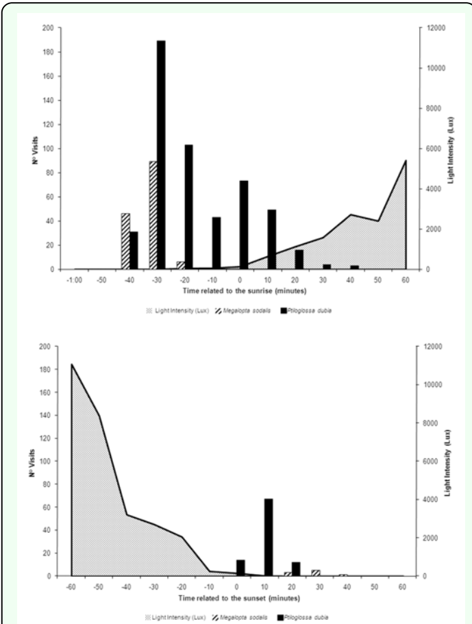
Figure 3. Number of visits of Megalopta sodalis and Ptiliglossa aff. dubia to Cambessedesia wurdackii flowers in relation to the time of sunrise (top) and sunset (bottom) (at time = 0) during the months of May 2008 and June 2008, and the corresponding light intensity values in an area of campo rupestre vegetation in Mucugê, Bahia State, Brazil. High quality figures are available online.
