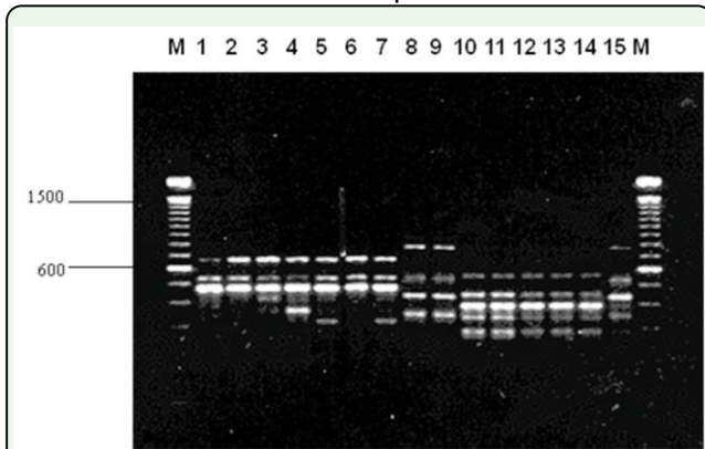
Figure 3. Representative gel comparing RAPD profiles between individuals of different stages of Cochliomyia hominivorax (lanes 1–7) with C. macellaria (lanes 10–15) using primer OPB-1. Lanes: (1–2) (CR92; Costa Rica) eggs, (3–4) first instar, (5) third instar, (6) pupa, (7) adult, (8–9) C. macellaria (CMN; Nebraska) eggs, (10–11) first instar, (12) third instar, (13–14) pupa, (15) adult. Lane M contains 100 bp ladder markers. High quality figures are available online.
