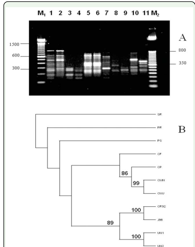
Figure 4. (A) Representative gel comparing RAPD profiles of individual unknown first instars from Nicaragua with first instars of Cochliomyia hominivorax in lanes (1) CR92 (Costa Rica) and (2) J98 (Jamaica) and other flies using primer OPA-12 (3–4) CMN ( C. macellaria ), (5–6) UNK, (7) CF, ( Chrysomya ruffacies ) (8) CP ( Calliphora vicina ), (9) PR ( Phormia regina ), (10) PS ( Lucilia sericata ), (11) SR ( Sarcophaga sp. ). Lanes M1 and M2 contain 100 bp and 50 bp ladder markers, respectively. (B) Dendrogram of the relationships between unknowns (UNK) from Nicaragua with screwworms and other flies from all gels and all scorable RAPD bands amplified from primer OPA-12, OPB-1, OPE-3 and OPE-14. Abbreviations same as for A above. Similarity values calculated by Nei-Li's coefficient; unweighted pair-group method using arithmetic averages clustering; only bootstrap values > 50% reported. High quality figures are available online.
