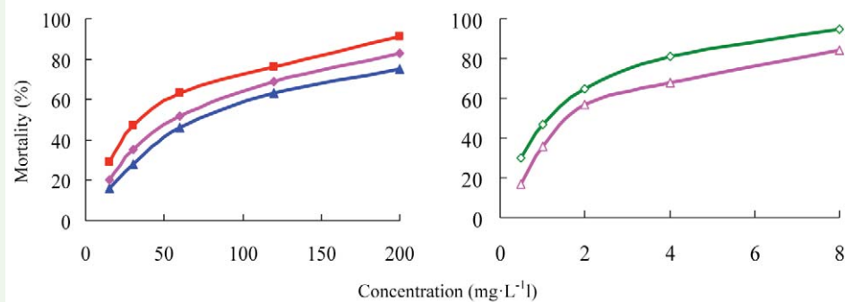
Figure 7. Concentration-response curves of etoxazole and other insecticides against Aphis craccivora (resistant). 99% etoxazole ( \Delta ), 5% etoxazole EC ( \diamond ), 95% permethrin ( \blacksquare ), 95% acephate ( \blacktriangle ), and 30% acephate EC ( \star ). High quality figures are available online.
