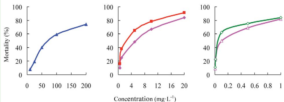
Figure 9. Concentration-response curves of etoxazole and other insecticides against Tetranychus cinnabarinus nymphs (resistant). 99% etoxazole ( \Delta ), 5% etoxazole EC ( \diamond ), 5% hexythiazox EC ( \blacksquare ), 98% clofentezine ( \blacktriangle ), and 98% hexythiazox ( \circ ). High quality figures are available online.
