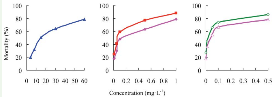
Figure 10. Concentration-response curves of etoxazole and other insecticides against Tetranychus cinnabarinus eggs (susceptible). 99% etoxazole ( \Delta ), 5% etoxazole EC ( \diamond ), 5% hexythiazox EC ( \blacksquare ), 98% clofentezine ( \blacktriangle ), and 98% hexythiazox ( \circ ). High quality figures are available online.
