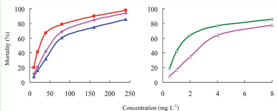
Figure 3. Concentration-response curves of etoxazole and other insecticides against Spodoptera exigua (resistant). 99% etoxazole ( \Delta ), 5% etoxazole EC ( \diamond ), 97% hexaflumuron ( \blacksquare ), 98% chlorfluazuron ( \blacktriangle ), and 5% chlorfluazuron EC ( \blacklozenge ). High quality figures are available online.
