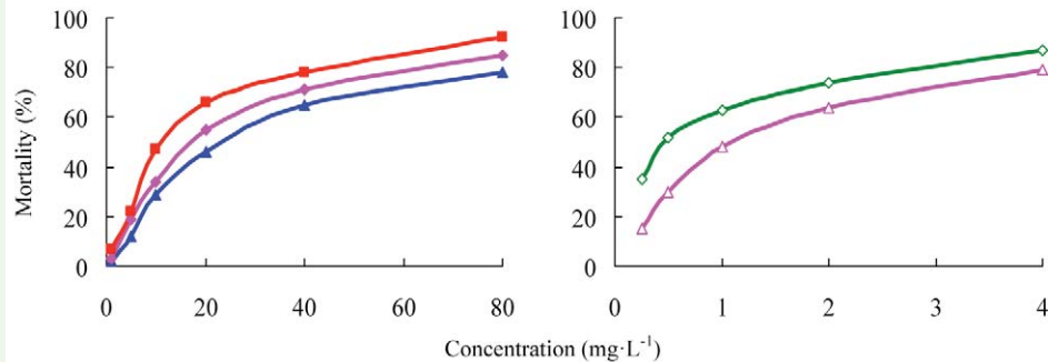
Figure 6. Concentration-response curves of etoxazole and other insecticides against Aphis craccivora (susceptible). 99% etoxazole ( \Delta ), 5% etoxazole EC ( \diamond ), 95% permethrin ( \blacksquare ), 95% acephate ( \blacktriangle ), and 30% acephate EC ( \star ). High quality figures are available online.
