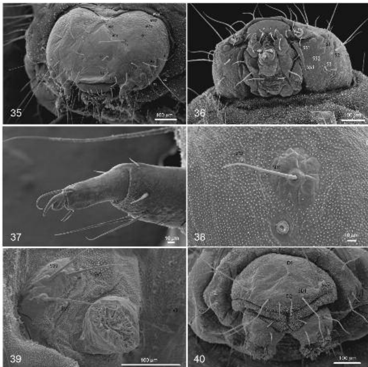
FIGS. 35–40. Gnoringoschema shepherdiae , scanning electron micrographs of larva. 35. Head chaetotaxy, frontal view. 36. Head chaetotaxy, ventral view. 37. Right tarsus on T2. 38. SD1 and SD2 on A5, right side. 39. Right proleg on A5. 40. Anal plate chaetotaxy on A10.
