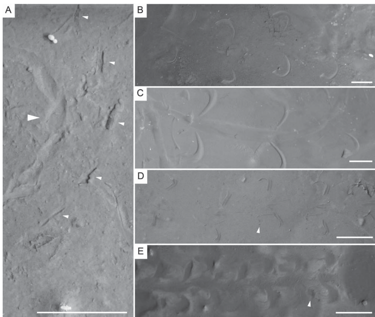
Fig. 6. Experimentally produced trackways; A: trackway produced by Notonecta sp. in soft mud. The segmented medial furrow is indicated with a large arrowhead whereas individual tracks are indicated with small arrowheads; B: trackway produced by Hesperocorixa sp. in soft mud under ~3.3 mm water; C: trackway produced by Hesperocorixa sp. in soft mud under ~3.5 mm water. D: trackway produced by Graphoderus liberus in firm mud under ~3.6 mm water; note the small imprints made by another set of appendages (one is arrowed) on both sides; E: trackway produced by Graphoderus liberus in soft mud under a film (ca. 1 mm) of water with small imprints again arrowed; Animal in A moved toward bottom of figure; all others moved from right to left. – Scale: 5 mm.
