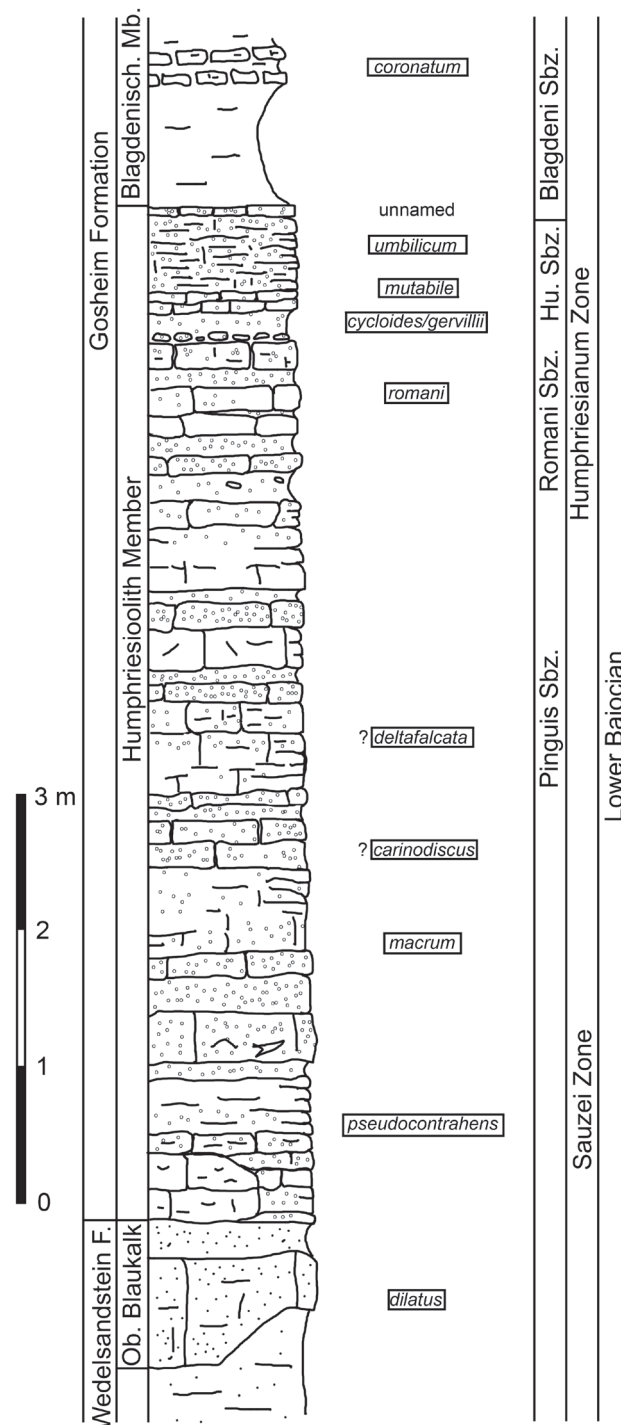
Fig. 2. Combined and slightly idealized section from the ‘Oberer Blaukalk’ Member up to the basis of the ‘Blagdenischichten’ at Gosheim (SW Germany) (based on OHMERT 1990, fig. 7 and own observations). Abbreviations: Wedelsandstein F. = Wedelsandstein Formation; Ob. Blaukalk = ‘Oberer Blaukalk’ Member; Blagdenischichten Mb. = ‘Blagdenischichten’ Member; Sbz. = Subzone; Hu. = Humphriesianum.
