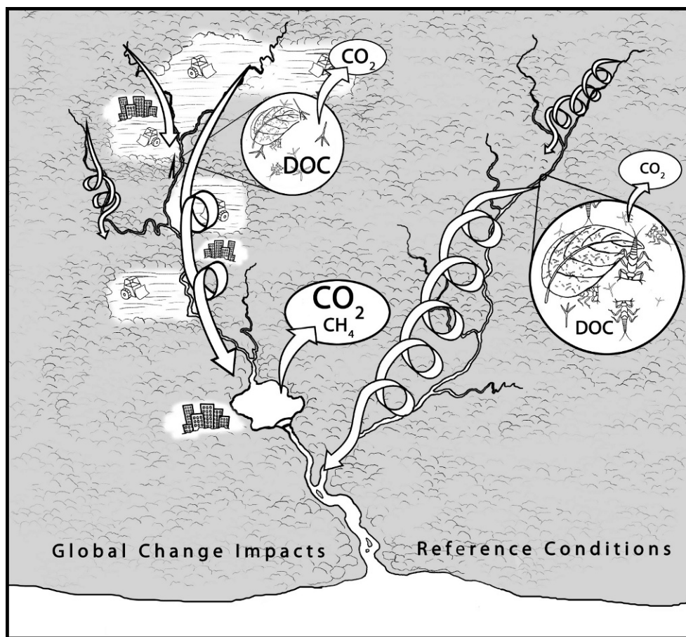
FIG. 2. Predicted interactive effects of drivers of global change on dynamics of organic matter in aquatic food webs and along river networks. Under reference conditions (right), terrestrially derived detritus is retained in situ and processed (multiple spirals in arrow indicating uptake, retention, and transformation) along river networks and supports high metazoan biomass. Drivers of global change (left) are predicted to reduce inputs and decrease retention (direct arrow) of organic matter with fewer opportunities for uptake and transformation (fewer spirals in arrow). Accumulation of particulate organic matter (POC) in reservoirs will increase reach- and network-scale losses of \text{CO}_2 and \text{CH}_4 relative to retained POC. Increased temperature and nutrient availability will promote greater microbial vs metazoan processing of organic matter (insets with leaves) and losses associated with respiration and greater leaching of dissolved organic C (DOC). Illustration credit: © Elizabeth Nixon 2010.
