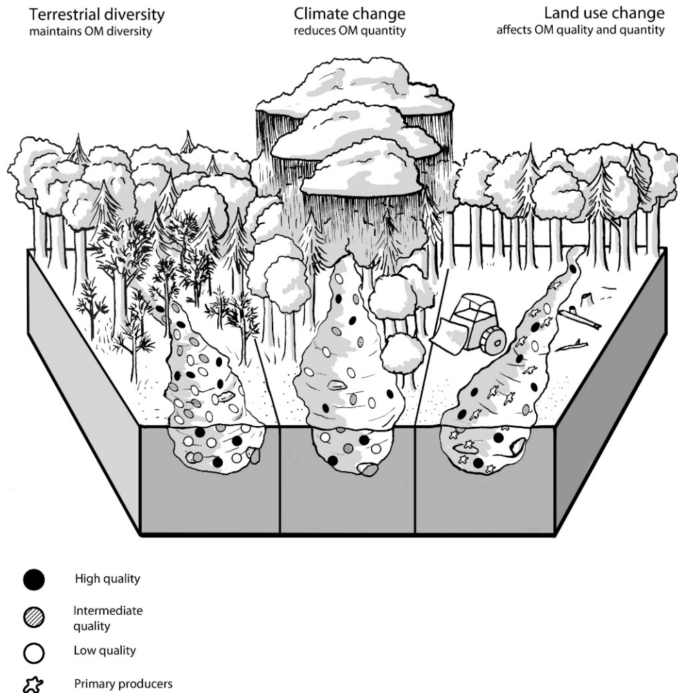
FIG. 1. Conceptual diagram of the net effects of drivers of global environmental change (biodiversity, climate, and land use) on dynamics of organic matter in riverine ecosystems. Vegetated watersheds with high terrestrial biodiversity provide a balance of low-to-high-quality organic matter (left). Climate change (altered precipitation and rising temperatures) will reduce the quantity of organic matter by increasing losses to downstream export during floods and increased processing rates (center). Land use changes will reduce inputs of terrestrial organic matter and nutrients, resulting in lower quantity of higher-quality detritus and increased autotrophic production (right). OM = organic matter. Illustration credit: © Elizabeth Nixon 2010.
