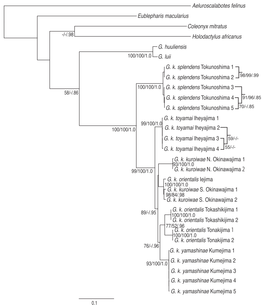
Fig. 2. Maximum-likelihood (ML) phylogeny of Goniurosaurus kuroi derived from 12S and 16S rRNA, and cytochrome b sequence data. Numbers below each node are bootstrap proportions (BPs) in 1000 replicates of ML and maximum parsimony (MP) analyses, and Bayesian posterior probabilities (BPPs) of eight million generations in Bayesian inference (BI), respectively. BP and BPP values smaller than 50% and 0.70, respectively, are omitted.
