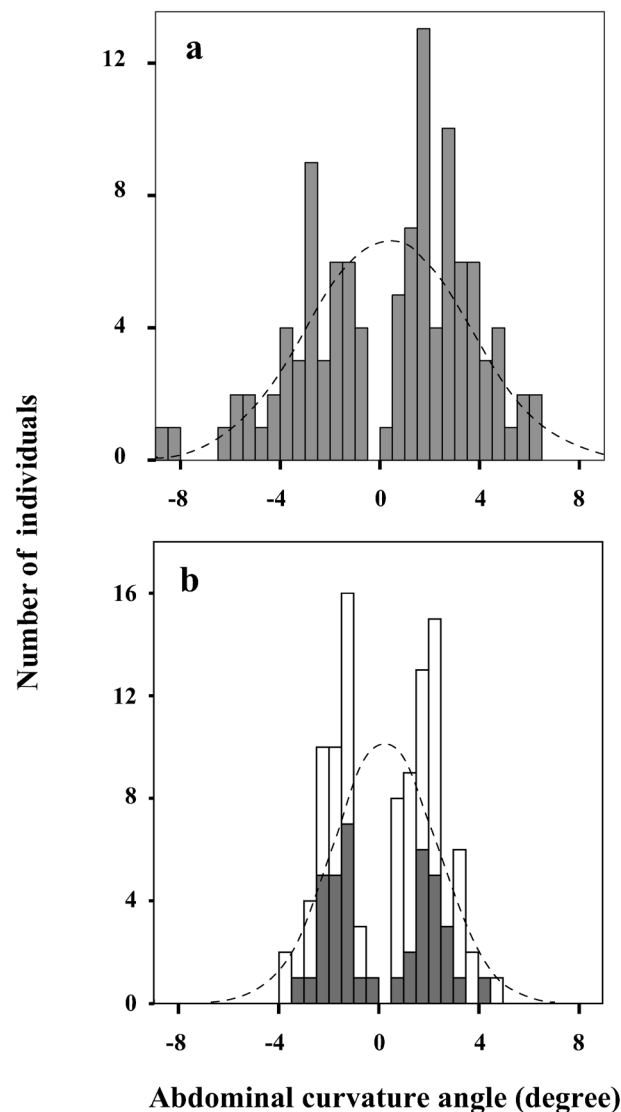
Fig. 3. Frequency distribution of the abdominal curvature angle of L. latipes (a) and N. denticulata (b) in each natural population. The dashed line indicates the normal curve fitted to the data. In N. denticulata , the dark column indicates males and the open column indicates females. The sexes of L. latipes individuals could not be determined.
