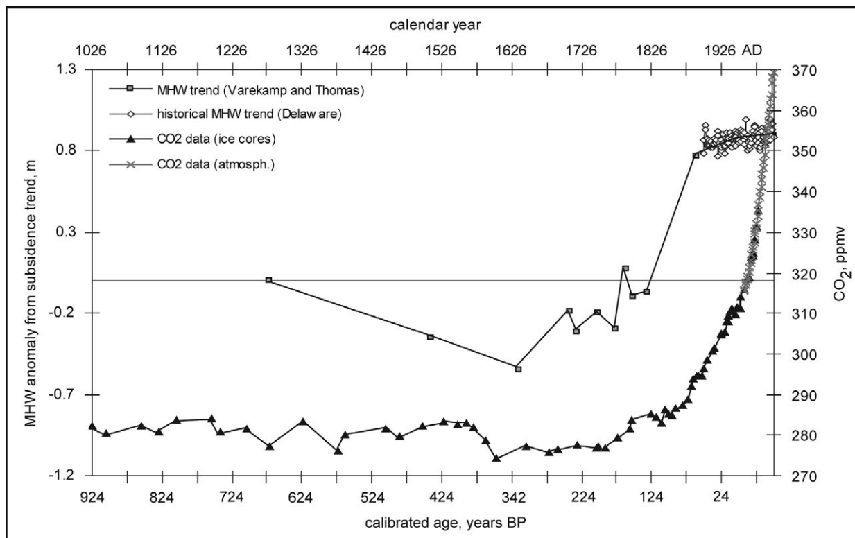
Figure 6. Comparison of \text{CO}_2 trends for the last millennium and MHW trends for Delaware Bay (Varekamp and Thomas, 1998, and historic record) adjusted for subsidence (2 mm/y).
