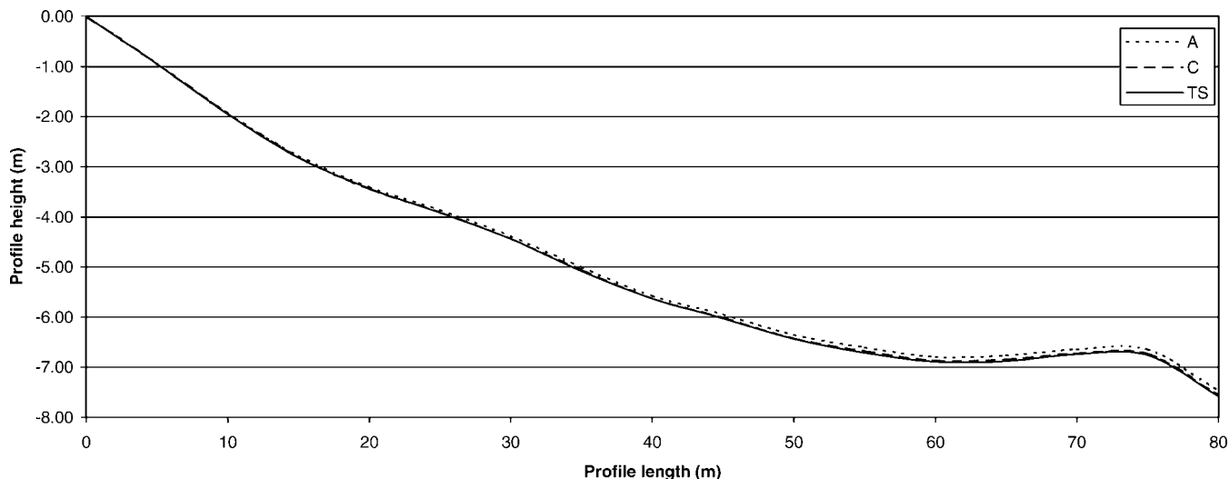
Figure 3. Comparison of beach profiles obtained with the proposed profiler (A and C) and with total station (TS). A relative profile height is presented as a negative value because it corresponds to vertical differences reported to the profile's anchor point.
