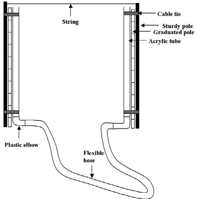
Figure 2. Sketch of equipment used for measuring beach profiles (profler): communicating vessel (hose, two plastic elbows, and two transparent acrylic tubes), two graduated poles, and, if necessary, two gardening poles for added robustness and stability.
