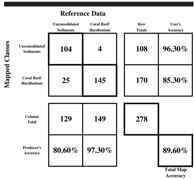
Figure 7. Confusion matrix for two generalized mapped classes: unconsolidated sediment and coral reef-hard bottom.
