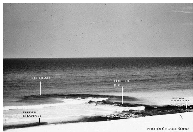
Figure 6. A rip current at Panama City Beach as marked by tracer dye is sinuous in shape because of a strong longshore current (photo by Dr. Choule Sonu). If someone tried to escape the rip by swimming to the right, they would be pulled back into rip current.
