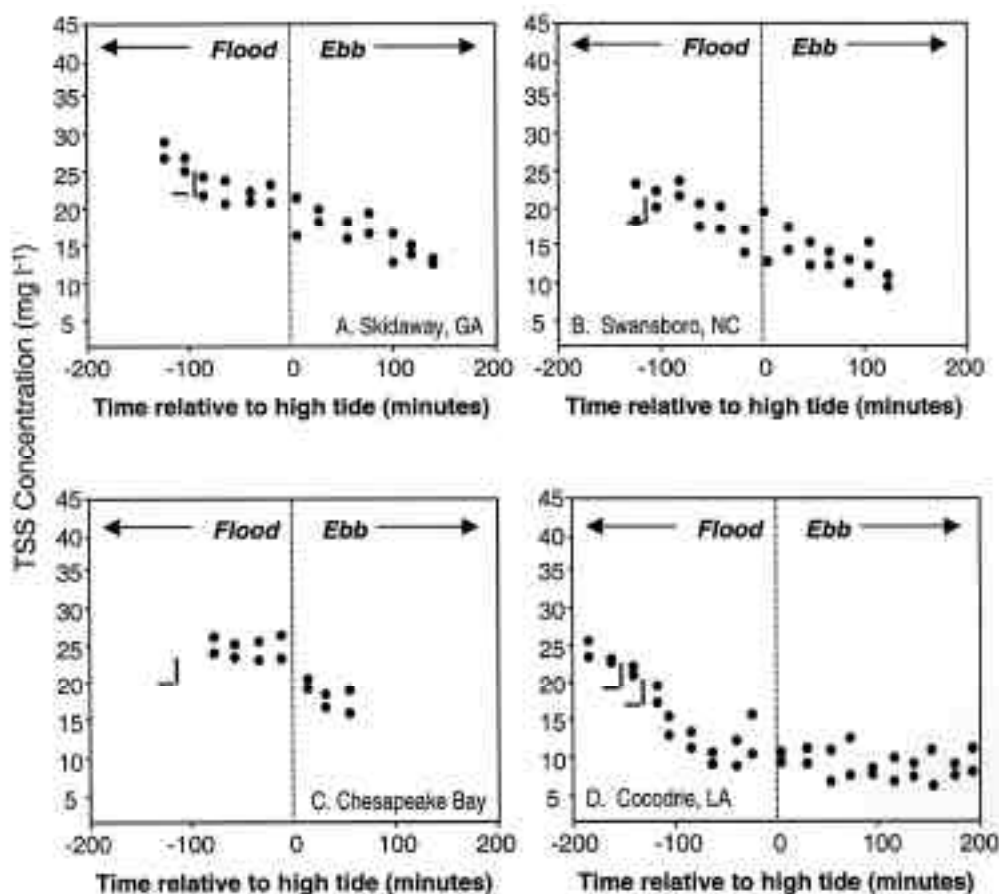
Figure 8. Figure 8. TSS concentrations measured on the surface of three semidiurnal marshes: A) Skidaway, GA (macrotidal), B) Swansboro, NC (low mesotidal), and C) Chesapeake Bay, MD (microtidal) and one diurnal marsh: D) Cocodrie, LA (microtidal). All data were collected at 5 cm above the bottom in S. alterniflora .
