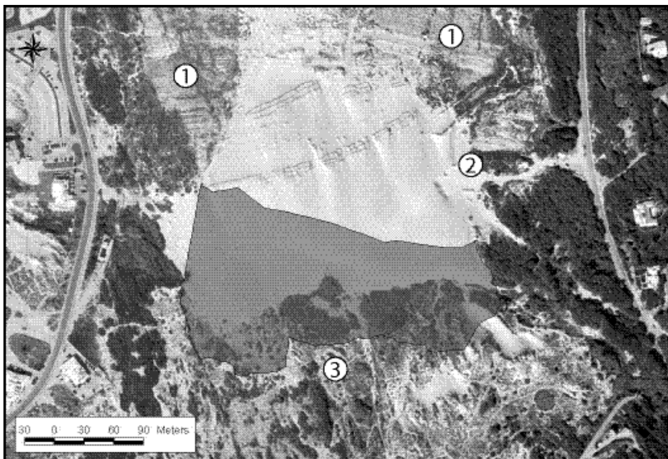
Figure 3 . Monitored area of 43067\text{m}^2 (grayish transparent layer) on top of the 2000's aerial photo. 1- Deflated area with exposed hardrock; 2 – Sand pit; 3 – Vegetated dunes.
