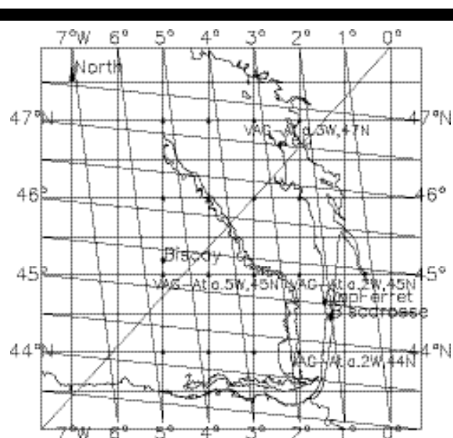
Figure 1 localization of data sources. The grid of output of the VAG-Atla model are shown by small diamonds. The position of wave riders are shown with greater diamonds. 4 isobathes are drawn: -50m, -200m, -400m, -1000m.
