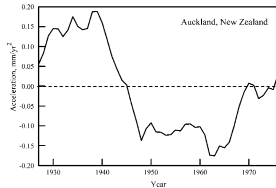
Figure 8. Sea-level acceleration at Auckland, New Zealand, based on 46-year records centered in years 1927–1976 and representing the years 1904–1998.
