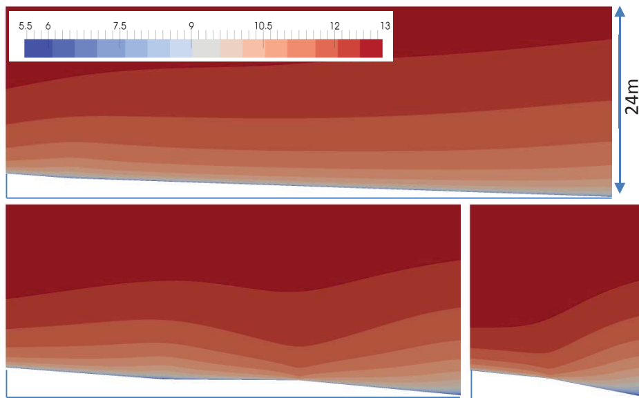
Figure 1. CFD generated velocity bands (scale bar in msec -1 ) across dissipative (Goolwa, uppermost), intermediate (Hawks Nest, lower left) and reflective beach (Jimmys) profiles illustrating minimal flow disturbance across the majority of the dissipative profile compared to the intermediate and reflective beaches. Horizontal distances are 80m, 60, 23m respectively (see fig 2). Wind flow is from right to left (and in the following diagrams).
