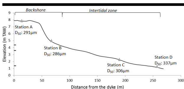
Figure 3. Sediment characteristics across the beach topography. Top, middle and bottom ticks on the y-axis correspond to the spring high water level, the maximum water level reached over the experiment, and the spring low water level respectively.
