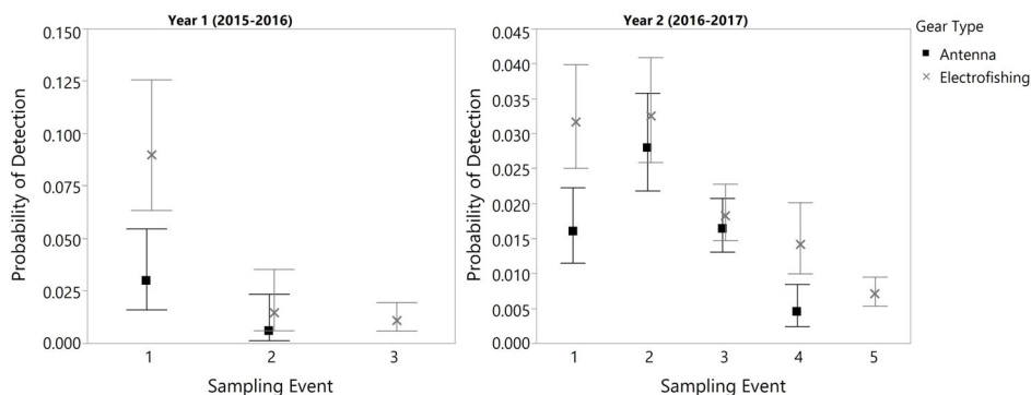
Figure 2. Probability, with 95% confidence intervals, of detecting passive integrated transponder (PIT) tagged roundtail chub ( Gila robusta ) by tow-barge electrofishing or portable, flat-bed PIT antennas after two stocking events in the upper Verde River, Arizona. Because methods changed slightly between each sampling year, data were grouped into discrete sampling events and gear types compared by year. Sampling events correspond with days post-stocking (e.g., Year 1 sampling events 1, 2, and 3 correspond with electrofishing surveys at 19, 26, and 83 days post-stocking, and Year 2 sampling events 1, 2, 3, 4, and 5 correspond with electrofishing surveys at 2, 16, 25, 52, and 85 days post-stocking). Note, x and y axes scales differ between sampling years, and antenna data are not present for the last sampling event in each year because antennas were removed prior to the last electrofishing survey.
