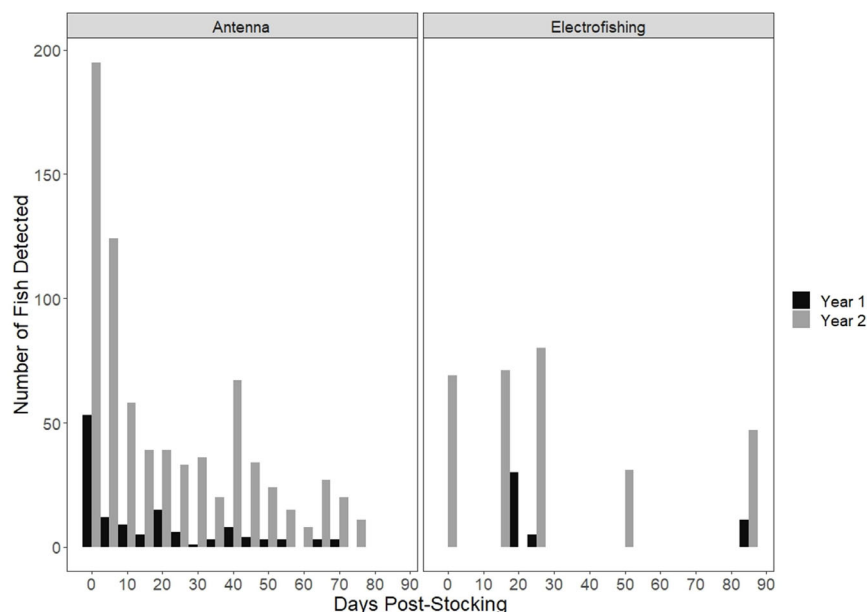
Figure 1. Number of individual roundtail chub ( Gila robusta ), detected by passive integrated transponder (PIT) antenna arrays or electrofishing surveys for each year after stocking in the upper Verde River, Arizona. In Year 1 (2015-2016) of sampling, 152 of 333 fish initially stocked were detected. Antennas detected 128 fish, while 46 fish were captured through electrofishing surveys. In Year 2 (2016-2017) of sampling, 893 fish were detected of the 2,177 fish initially stocked. Antennas detected 750 fish, while 298 fish were captured through electrofishing surveys.
