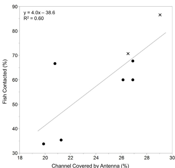
Figure 4. Linear relationship of channel coverage (%) and PIT tagged roundtail chub ( Gila robusta ) contacted (%) for both small rectangular (Marsh & Associates, LLC, Tempe, AZ, 0.9 m length x 0.7 m height) and large rectangular (Marsh & Associates, LLC, Tempe, AZ, 1.3 m length x 0.7 m height) PIT antennas in the upper Verde River, Arizona. Small antennas are denoted with a circle and large antennas are denoted with an "X". Note that the x and y scales do not begin at zero. The variation in the percent of tagged roundtail chub contacted can be explained by channel coverage, which is the physical area covered by an antenna. Generally, antennas that spanned a larger portion of the channel contacted more tagged roundtail chub.
