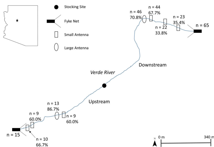
Figure 3. Small (Marsh & Associates, LLC, Tempe, AZ, 0.9 m length x 0.7 m height) and large (Marsh & Associates, LLC, Tempe, AZ, 1.3 m length x 0.7 m height) rectangular passive integrated transponder (PIT) antenna and fyke net locations in the upper Verde River, Arizona, in Year 2 (2016-2017) of the study. Numbers of hatchery-reared, PIT tagged roundtail chub ( Gila robusta ) captured by fyke nets and contacted by antennas within 72-h of stocking are represented next to the associated symbol. Detection efficiency of individual antennas are represented in percentages.
