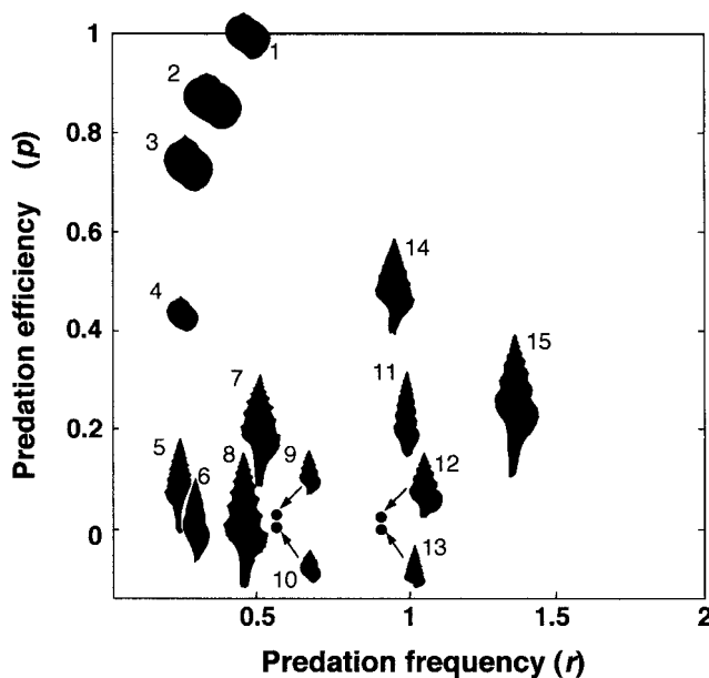
Figure 5. Predation efficiency ( p ) and predation frequency ( r ) for 15 gastropod species from Shinzato Formation. Data from Table 1. Abbreviations: 1, Naticolius cf. niasensis ; 2, Natica sp.; 3, Natica aff. stellata ; 4, Euspira cf. pallida ; 5, Gemmula cassinella ; 6, Daphnella ryukyuensis ; 7, Coronasyrinx takabanarensis ; 8, Gemmula granosa ; 9, Hindsia takabanarensis ; 10, Cancellaria yonabaruensis ; 11, Splendrillia sp.; 12, Hindsia solida ; 13, Trochocerithium shikoensis ; 14, Makiyamaia coreanica ; 15, Pseudo-litirus yonabaruensis .
