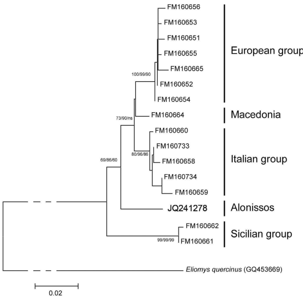
Fig. 2. Neighbor-joining tree of haplotypes of the edible dormouse. The specimen from Alonissos is indicated in bold. Numbers at nodes specify bootstrap values at NJ /MP/ ML. Only basal nodes with values higher than 50 % are indicated.
