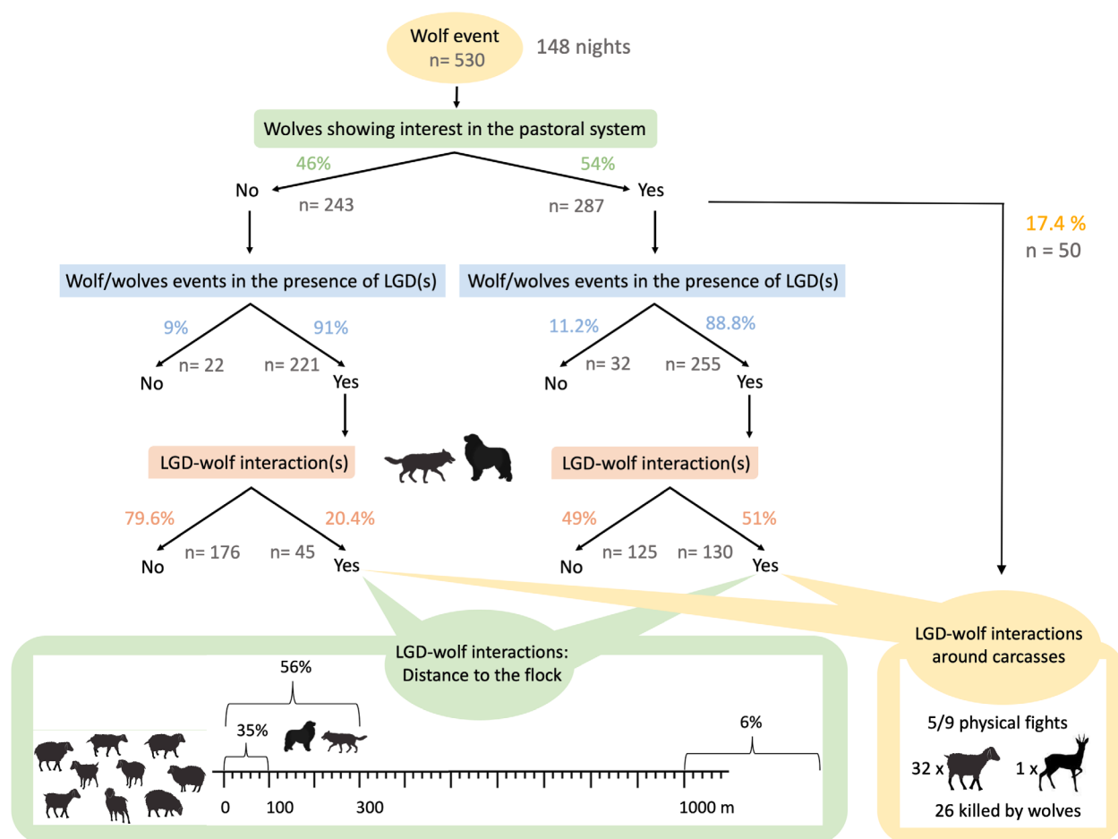
Fig. 2. Hierarchical diagram summarizing how wolf events lead to interactions between livestock guarding dogs and wolves, the distance of these interactions from the flock and the special case of carcasses present on pastures in the southern French Alps.
