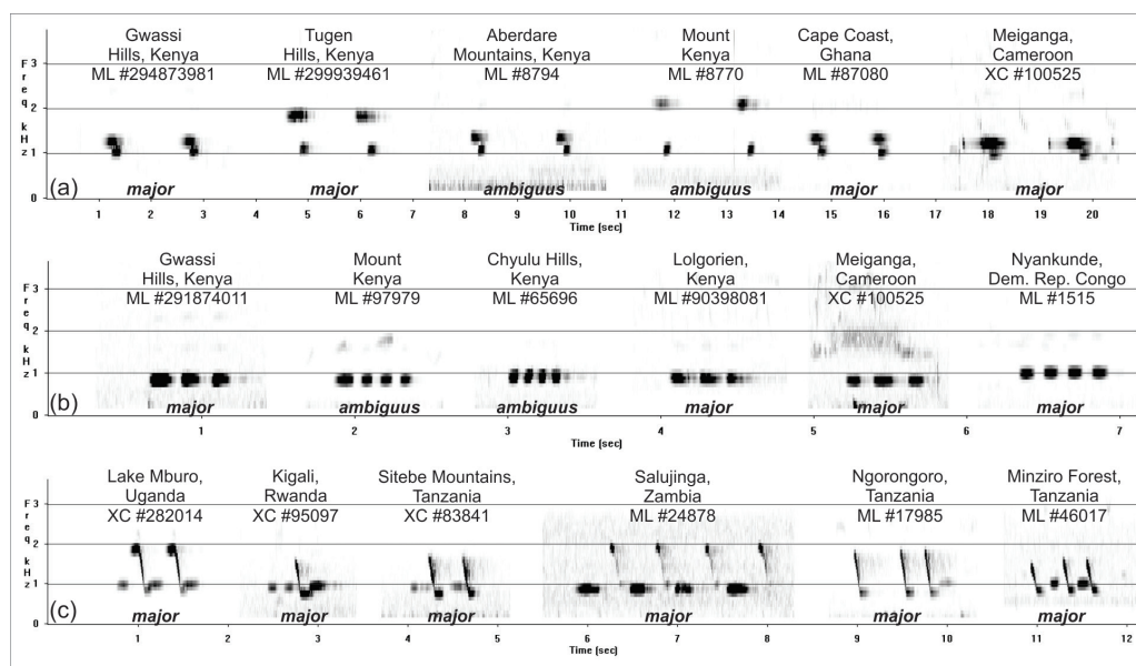
Figure 1. Sonograms of the Tropical group showing (a) variation in the basic tee-loo high-low duet (one motif repeated once), (b) rapid, multiple bell-note too-too-too calls of Tropical Bouobou Laniarius major and L. m. ambiguus from West Africa to Kenya (single bird), and (c) varying-pitch notes with gonolek-like quality in duets of L. major from south-west Uganda, Zambia, and the Mufindi and Ngorongoro regions of Tanzania. For recording credits see Appendix.
