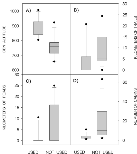
Figure 1. Box plots, showing median, lower and upper quartiles (box), 10 and 90% quartiles (intervals) and sample minimum and maximum, for the relationship between arctic fox den use in Børgefjell and A) den altitude (in m a.s.l.), B) kilometres of trails, C) kilometres of roads and D) number of cabins. The three infrastructure variables were measured within squares of 15 \times 15 km with the den in the centre. For each predictor, the box to the left gives the values for dens used ( N=14 ) whereas the box to the right gives the values for dens not used ( N=13 ) during 2001-2005.
