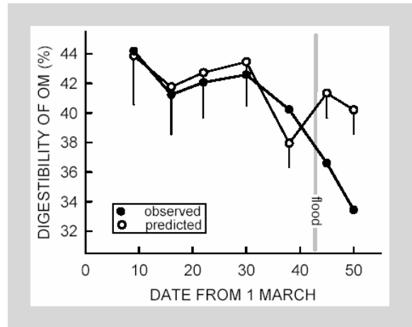
Figure 2. Apparent digestibility of organic matter of barnacle geese in large pens on Festuca swards. Observed digestibilities, based on ADF as a natural marker, are compared with predictions from indoor feeding trials (mean \pm 1 SE, based on the regression in Table 2). The vertical line indicates when the salt marshes were flooded during high tides.
