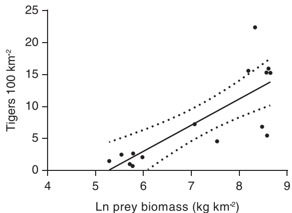
Figure 2. Relationship between tiger density and biomass of important ungulate prey for 15 areas in Asia. The relationship is described by the equation: tiger density = 4.1012 Ln (preferred ungulate biomass) - 21.626; R^2 = 0.61507 .
