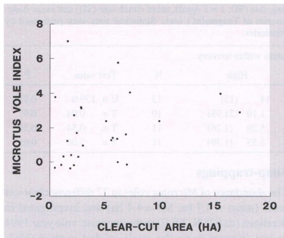
Figure 1. Microtus vole density expressed as the number snap-trapped per 100 trap-nights in relation to clear-cut areas (N = 27) in the 'increase' vole year 1994. Jitter-option (Sygraph drawing program) was used to separate overlapping datapoints.
