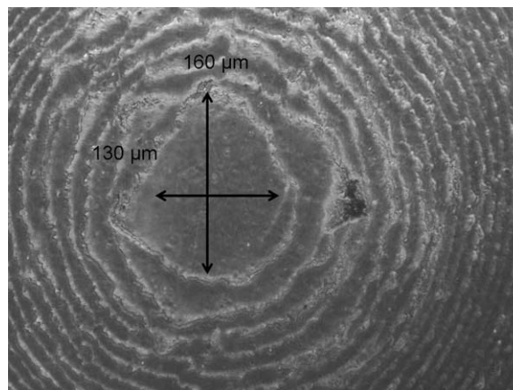
Figure 3. Eye lens nucleus of Enteroctopus megalocyathus from a polished surface of plastic resin embedding under phase contrast microscopy (400 \times ).
