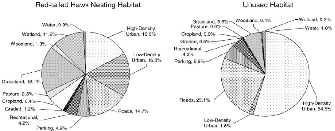
Figure 2. Land-cover composition for urban/suburban Red-tailed Hawk nesting habitat and unused habitat within the Metropolitan Milwaukee Study Area (MMSA).
