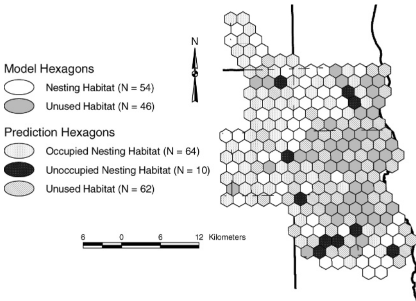
Figure 4. Predictions of the Red-tailed Hawk nesting habitat model.
