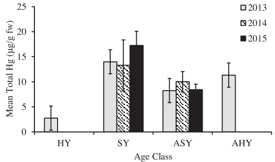
Figure 3. Concentrations of mean total mercury ( \mu\text{g/g} fresh weight) detected in fourth primary feathers collected from migrating Peregrine Falcons captured at South Padre Island, Texas, during autumn migrations in 2013–2015. Arithmetic means are presented with standard error bars. Years and age class categories are shown, with 117 hatch-year, 15 second-year (SY), 44 after-second-year (ASY), and 11 after-hatch-year (AHY) peregrines sampled in 2013; 3 SY and 6 ASY sampled in 2014; and 8 SY and 17 ASY individuals sampled in 2015. Only those individuals older than HY and not identified more precisely by plumage were categorized as AHY.
