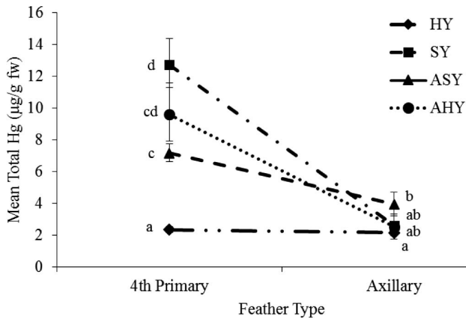
Figure 2. Concentrations of mean total mercury (THg; \mu\text{g/g} fresh weight) by age class detected in fourth primary and axillary feathers collected from migrating female Peregrine Falcons captured at South Padre Island, Texas, in autumn 2013. Back-transformed means with standard error bars of THg concentrations are shown from our mixed-effects ANOVA model including feather type and age as fixed effects. Letters next to each symbol indicate significant difference among means, determined using Tukey post-hoc differences <0.05 . Fourth primary feather sample size varied: 82 hatch-year (HY), 15 second-year (SY), 40 after-second-year (ASY), and 11 after-hatch-year (AHY). Axillary feather sample size also varied: 78 hatch-year (HY), 15 second-year (SY), 39 after-second-year (ASY), and 11 after-hatch-year (AHY). Only those individuals older than HY and not identified more precisely by plumage were categorized as AHY.
