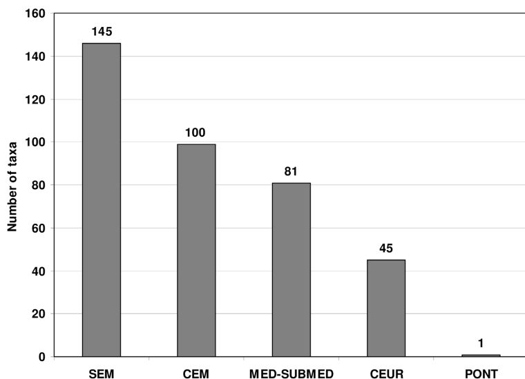
Fig. 4. Spectrum of chorological groups in the Balkan endemic vascular flora of Montenegro. – SEM: southern European mountain; CEM: central European mountain; MED-SUBMED: Mediterranean-submediterranean; CEUR: central European; PONT: Pontic.
