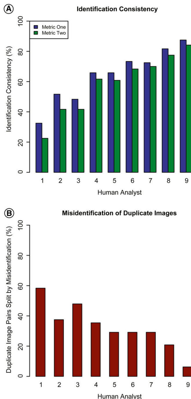
Fig. 3. Identification consistency of the nine analysts expressed using the two consistency metrics described in the main text (A), and as the percentage of duplicate image pairs that were split by misidentification (B).
