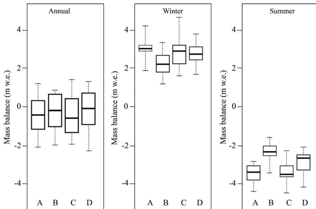
Figure 5. Box plots of surface mass balance measurements on four glaciers in and near the Skagit basin from 1993 to 2013 (A-Noisy, B- Silver, C-N. Klawatti, D-Sandalee). Dark horizontal lines represent average balance, boxes represent the interquartile range (25 to 75th percentiles), and dashed lines are 5–95 percentile range of values.
