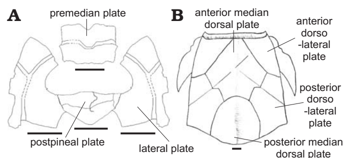
Fig. 12. Reconstructions of the dermal shield of antiarch placoderm Remigolepis durnalensis sp. nov., from Spontin (Namur Province), Famennian, Devonian. A. Reconstruction of the incomplete head shield (the left lateral plate is the mirror image of the right one), dorsal view. B. Trunk reconstruction, dorsal view. Scale bars 10 mm.
