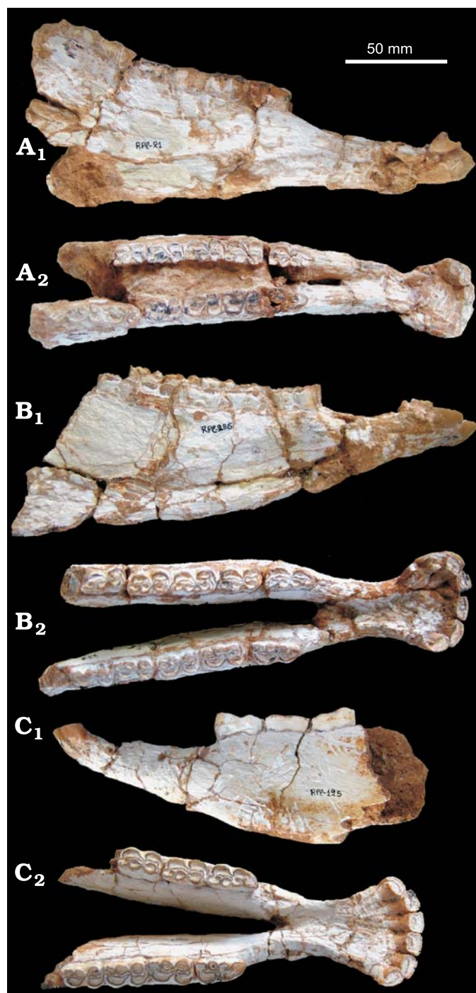
Fig. 3. Equid Hipparion macedonicum Koufos, 1984 from Ravin de la Pluie, Axios Valley (Macedonia, Greece), late Vallesian, MN 10 (Late Miocene). A. Holotype LGPUT RPI-21, mandible in right lateral (A 1 ) and occlusal (A 2 ) views. B. LGPUT RPI-286, mandible in right lateral (B 1 ) and occlusal (B 2 ) views. C. LGPUT RPI-125, mandible in left lateral (C 1 ) and occlusal (C 2 ) views.
